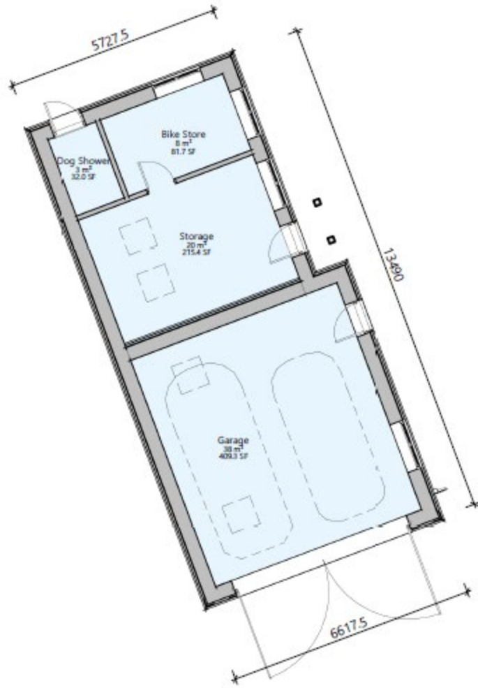
1 Garage Block - Ground Floor Plan 1 : 100
